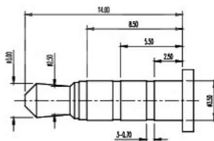
(#3.50mm 4 POLE PLUG DETAIL DRAWING)
