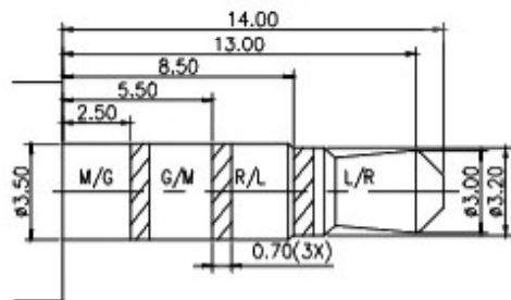
MATING PLUG
