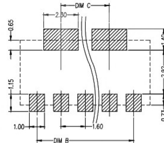
5-10PIN LAYOUT
