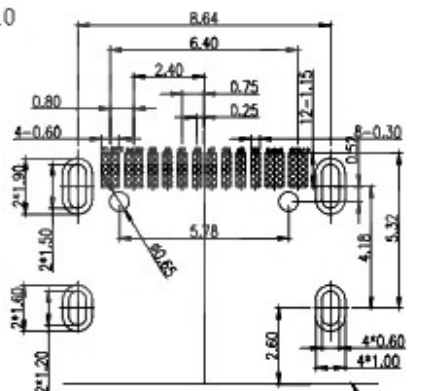
RECOMMENDED P.C.B. LAYOUT TOLERANCE UNSPECIFIED \pm 0.05\text{mm}
