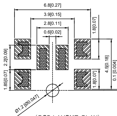
(PCB LAYOUT PLAN)
