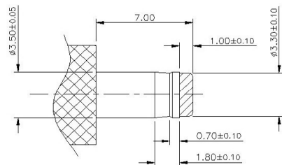
(ø3.50mm DC PLUG DETAIL DRAWING)
