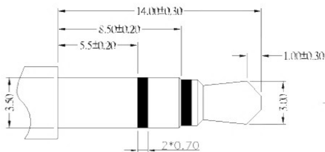
Ø3.50mm 3 POLE PLUG
