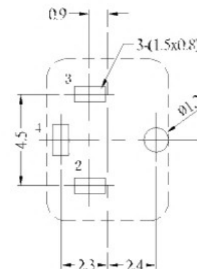
PCB LAYOUT MOUNTING PATTERN (TOP VIEW)
