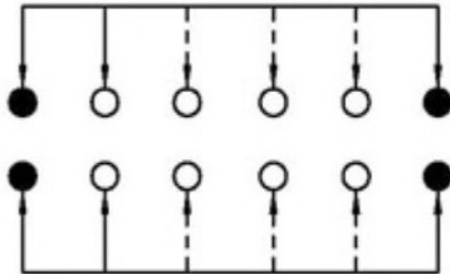
SCHEMATIC (NON-SHORTING)
