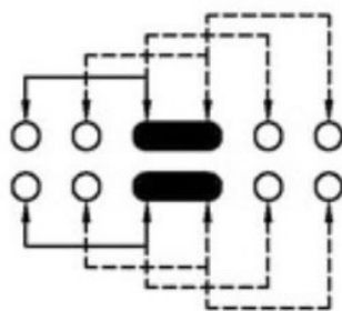
SCHEMATIC (SHORTING)
