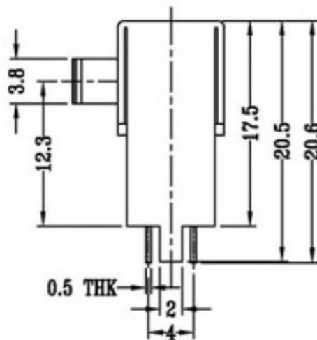
SCHEMATIC (SHORTING)
