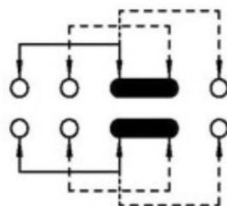
SCHEMATIC (SHORTING)
