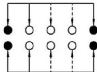
SCHEMATIC (NON-SHORTING)
