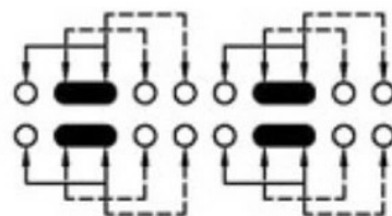
SCHEMATIC (SHORTING)
