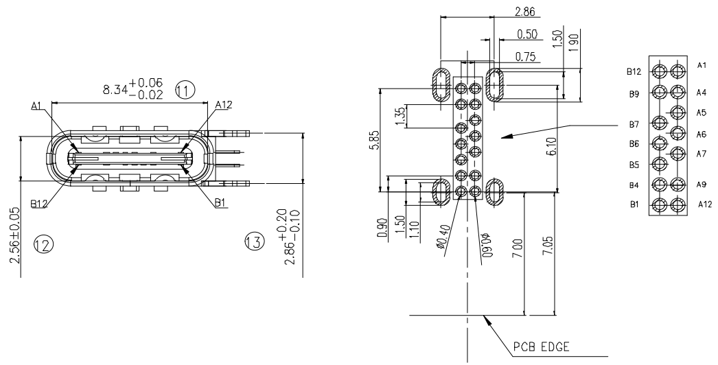
RECOMMENDED P.C.B. LAYOUT TOLERANCE UNSPECIFIED ±0.05mm
