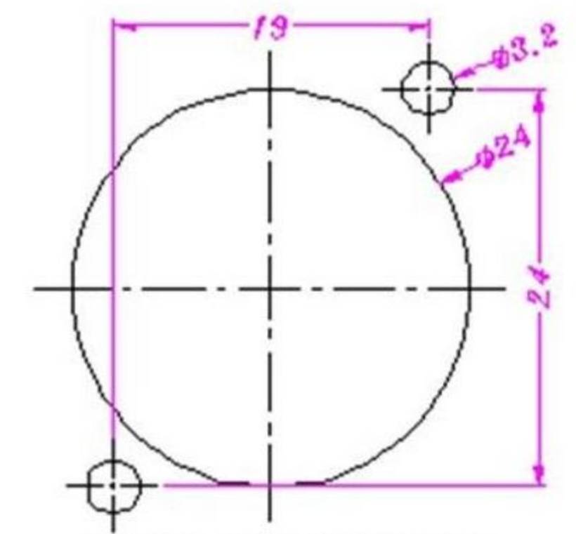
PANEL CUTOUT DETAIL
