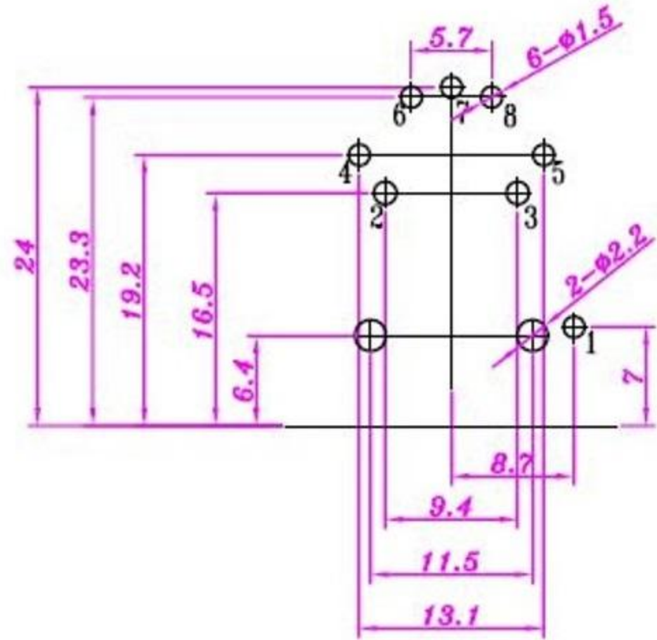
PCB LAYOUT
