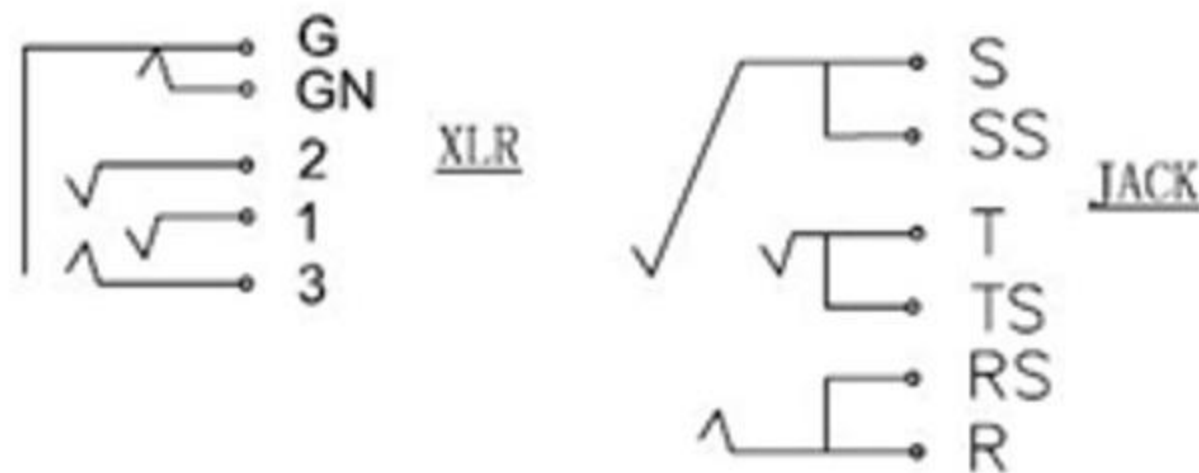
CONTACT SCHEMATIC CHART
