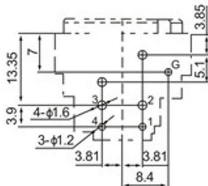
PCB LAYOUT (VIEWED FROM COPPER SIDE)
