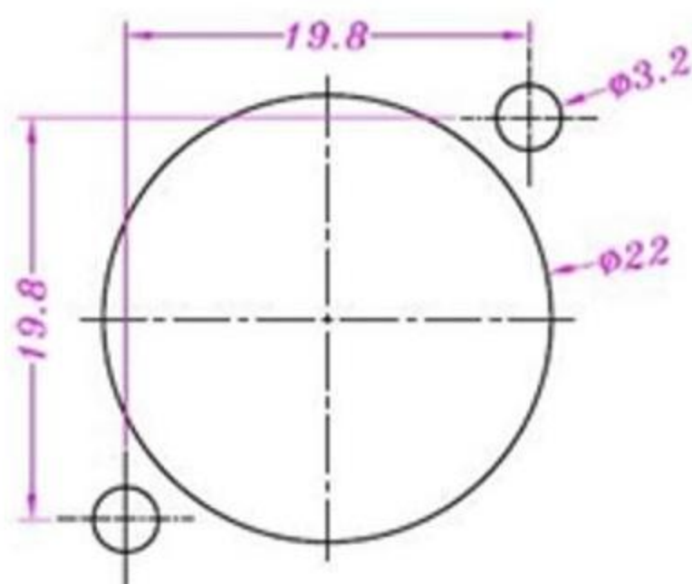
PANEL CUTOUT DETAIL
