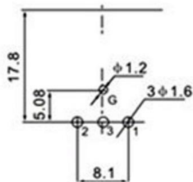
P.C.B LAYOUT (VIEWED FROM COPPER SIDE)
