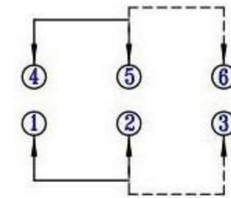
SCHEMATIC (NON-SHORTING)
