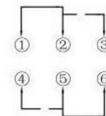
SCHEMATIC (NON-SHORTING)
