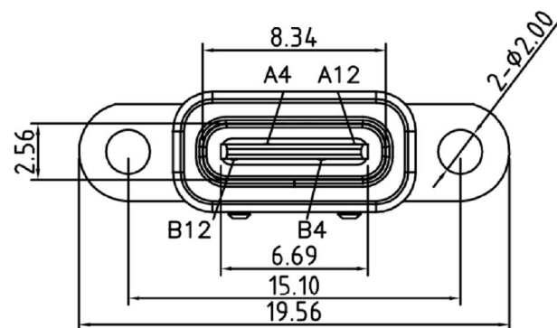
INTERFACE(FRONT VIEW)
