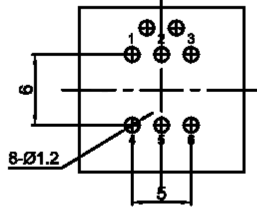
PCB HOLE(BOTTOM VIEW)
