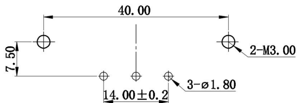
PCB LAYOUT
