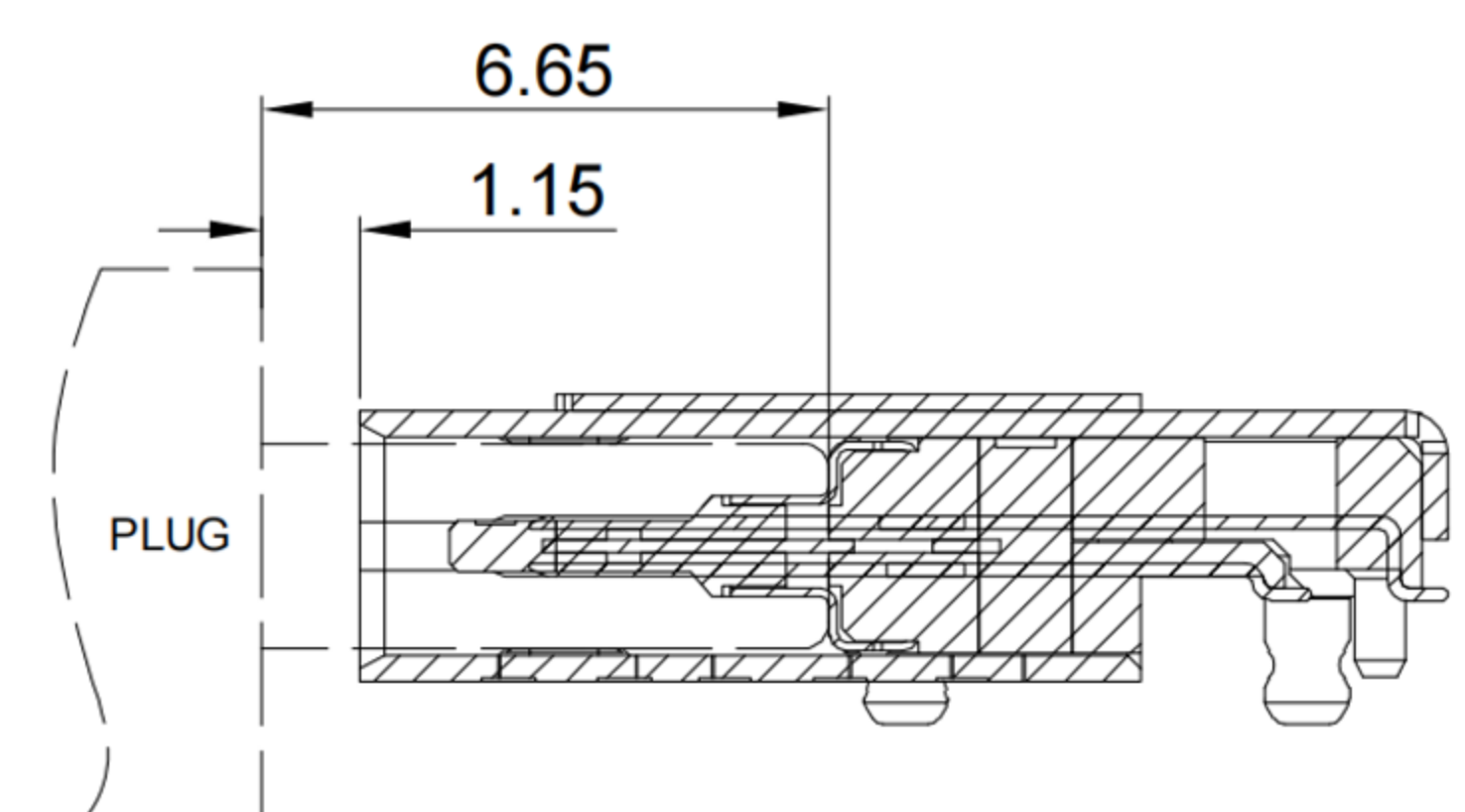
AFTER MATING(REF)
