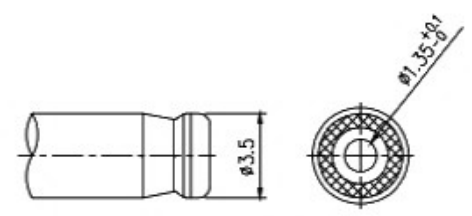
MATING PLUG \phi 3.50
