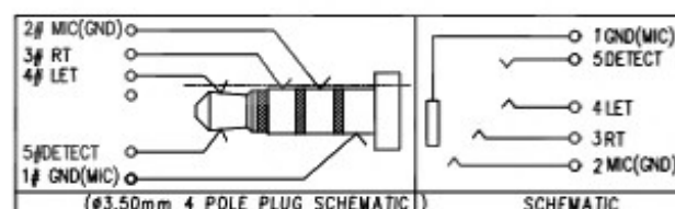
(#3.50mm 4 POLE PLUG SCHEMATIC)
