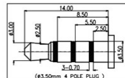
(#3.50mm 4 POLE PLUG)
