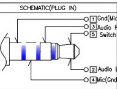
(Ø3.50mm 4 POLE PLUG DETAIL DRAWING)
