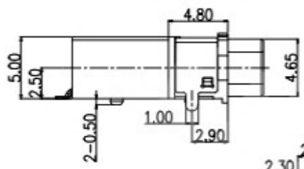
PLUG MATE DRAWING
