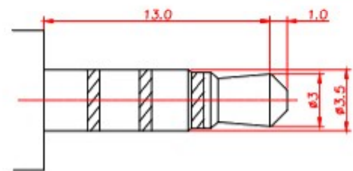
MATING PLUG
