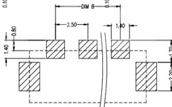
RECOMMENDED PCB LAYOUT TOL:(±0.05)
