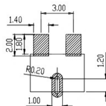
RECOMMENDED PCB LAYOUT TOL: ( \pm 0.05 )
