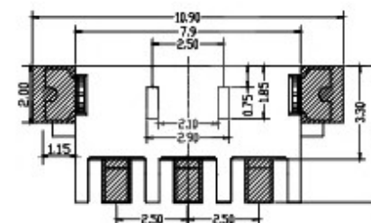
PCB LAYOUT (3pin)
