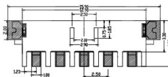
PCB LAYOUT (5pin)
