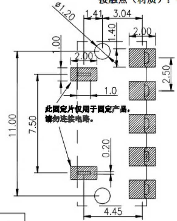
RECOMMENDED PCB LAYOUT TOP VIEW(. XX±0.05)
