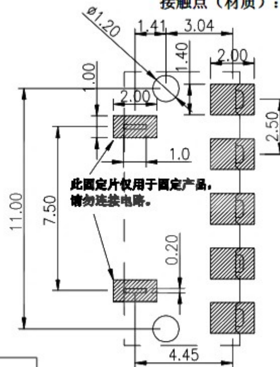
RECOMMENDED PCB LAYOUT TOP VIEW(. XX±0.05)
