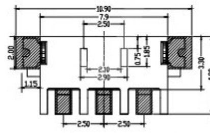
PCB LAYOUT (3pin)
