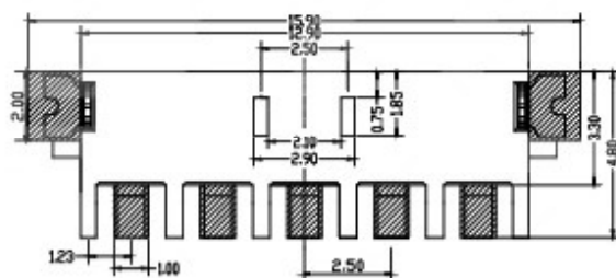
PCB LAYOUT (5pin)
