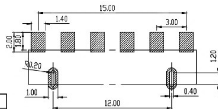
RECOMMENDED PCB LAYOUT TOL: ( \pm 0.05 )
