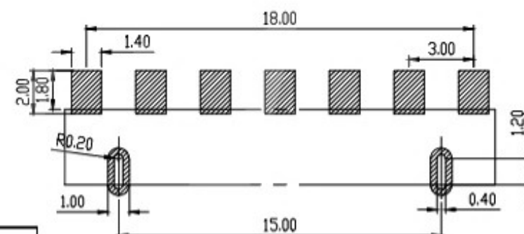
RECOMMENDED PCB LAYOUT TOL:(<±0.05)
