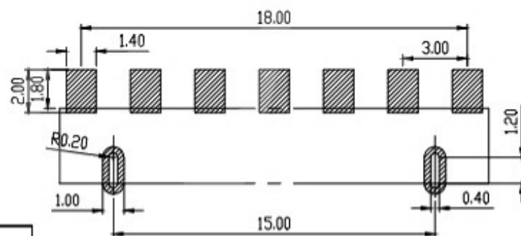
RECOMMENDED PCB LAYOUT TOL:(<math>\pm 0.05</math>)
