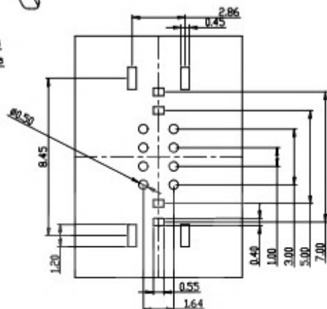
RECOMMENDED P.C.B. LAYOUT (T:1.00mm) TOLERANCE UNSPECIFIED ±0.05mm
