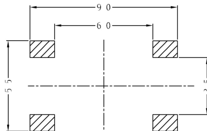
PCB LATOUT TOP VIEW
