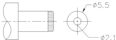
MATING PLUG Jack Insertion Depth: 9.0 mm
