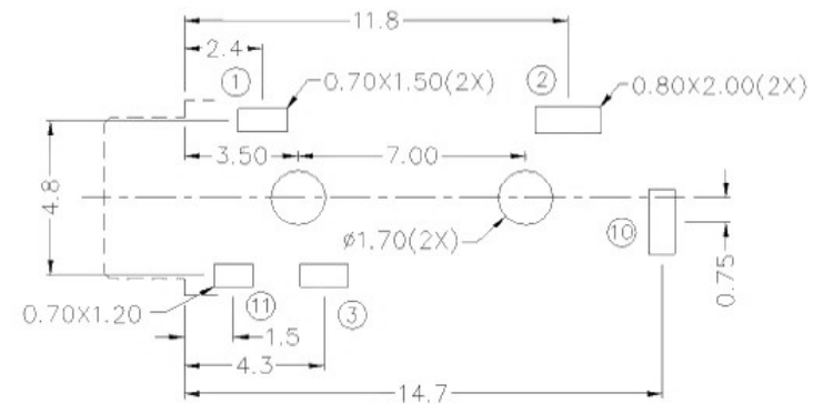
RECOMMENDED (BOTTOM VIEW)
