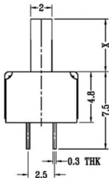
SCHEMATIC (NON-SHORTING)
