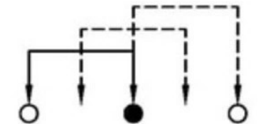
SCHEMATIC (NON-SHORTING)
