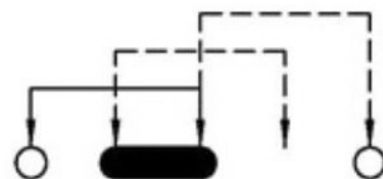
SCHEMATIC (NON-SHORTING)
