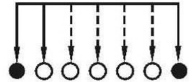
SCHMATIC (NON-SHORTING)
