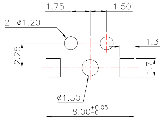
HOLE LAYOUT
