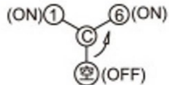
ON-ON-OFF SCHEMATIC (NON-SHORTING)
