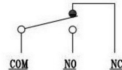
SCHEMATIC (NON-SHORTING)
